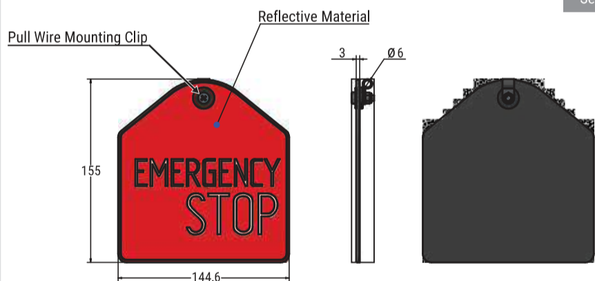
PULL WIRE MOUNTING SIGN Mass: 0.032 Kg
