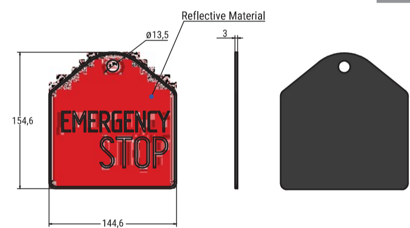
GUIDE MOUNTING SIGN Mass: 0.025 Kg
