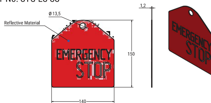
GUIDE MOUNTING SIGN Mass: 0.153 Kg
